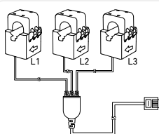
Current Transformer (×3)
